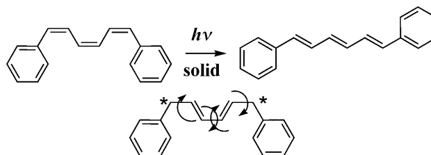
Scheme 2. The disrotatory double BP process in the S_1 stage of the ccc -DPH \rightarrow ttt -DPH photoreaction.
